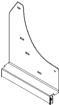
(1) Flap Assy Upper Rear, DS Part #770187
